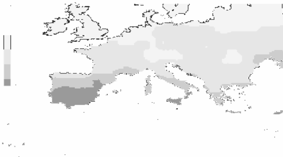
Figure III.5. Annual potential evapotranspiration map for Europe (EEA, 1996).
