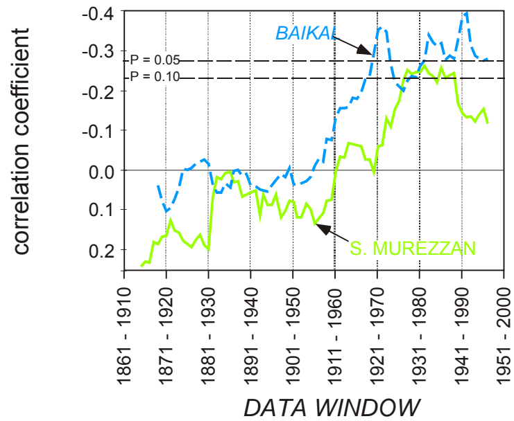
Figure IV.A.4. Running correlation of a 50 years time window between ice-break-up data from the lakes Baikal and San Murrezan and the NAO Index (modified from (Straile et al. 2003))
